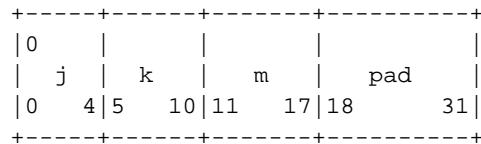
Figure 3-12. Boundary Alignment
