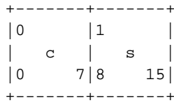
Figure 3-15. Union Allocation
