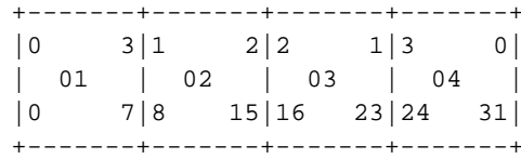
Figure 3-11. Bit-field Allocation
